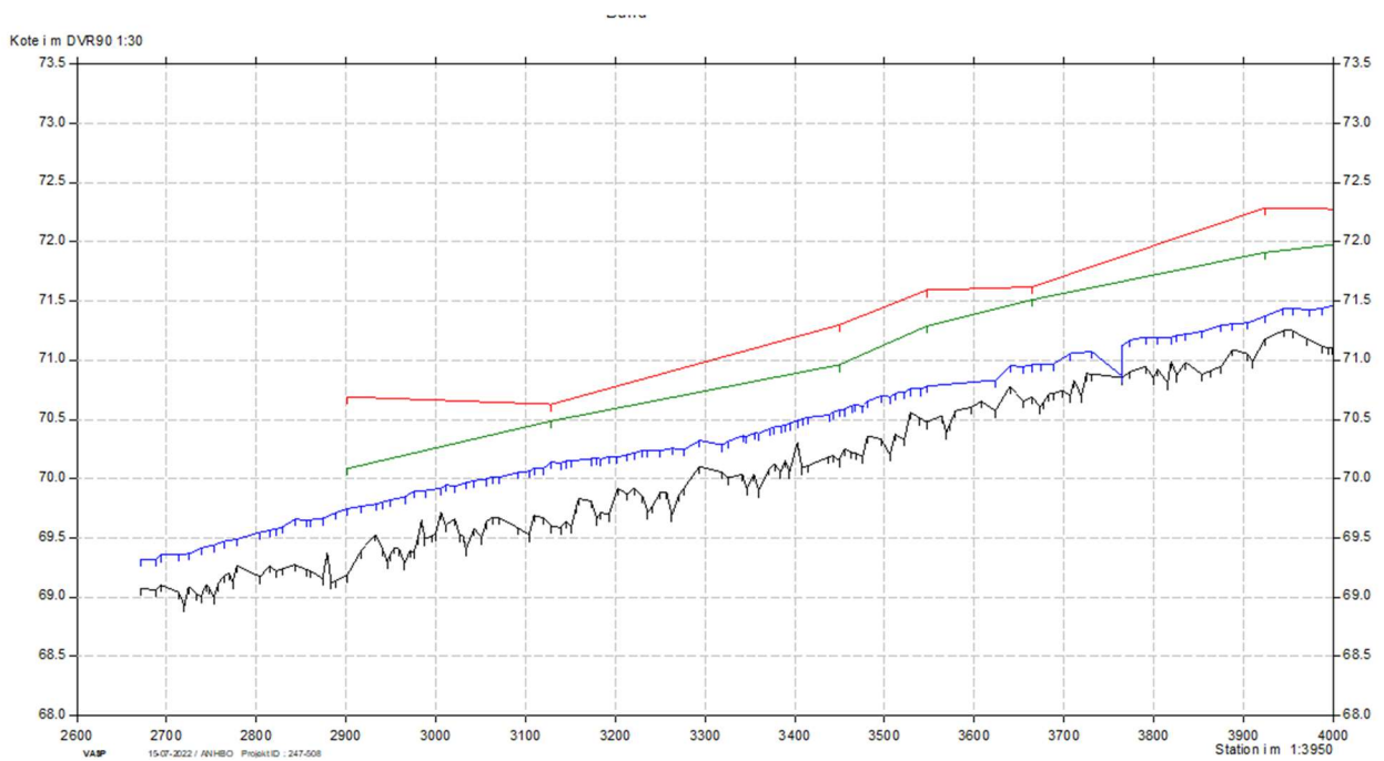
Figur 24 - stationering
